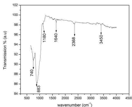
Fig.7:FTIR spectra of as deposited CdS film
